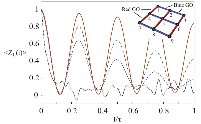
FIG. 1. (Color online) The expected value of the logical operator Z_L of the 3 \times 3 Bacon-Shor code. In the inset, each black sphere represents a physical qubit, and each (blue or red) bond represents a gauge operator (GO). The overall measurement is constructed by projectively measuring blue GOs first and then red GOs, and it is performed N times during the entire time of evolution \tau at equal interval. Here, the black dotted, blue short-dashed, green long-dashed, and red solid lines correspond N = 0, 500, 1000, and 5000 , respectively. In this simulation, a total of eight Hadamard gates are performed.
