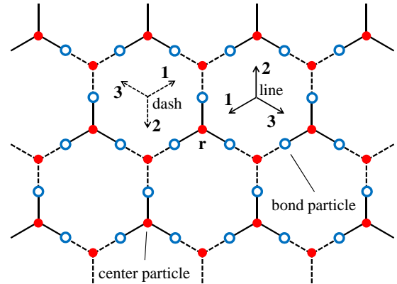
FIG. 1: The two-dimensional system composed of spin-3/2 particles. The system is a hexagonal lattice, where center particles (red round) are located on vertices, while bond particles (blue ring) are located on edges. There are two kinds of interactions between center particles and bond particles, V_{\text{line}} (line) and V_{\text{dash}} (dash line). \mathbf{r} denotes the position of a center particle, and the vectors between the center particle and its three interacting bond particles are \mathbf{1} , \mathbf{2} , \mathbf{3} respectively.
