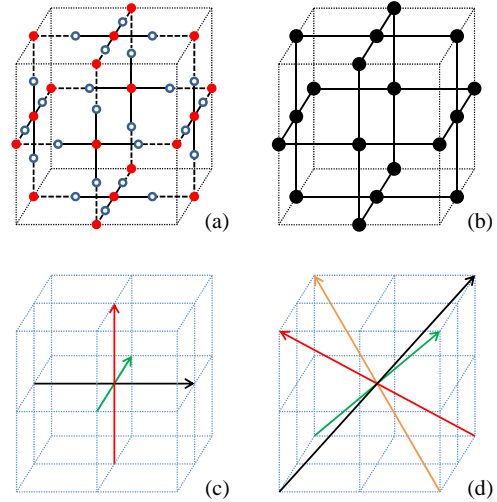
FIG. 2: The three-dimensional system. (a) The elementary cell of the system. The system is composed of spin-2 particles and spin-3/2 particles. Spin-2 particles are center particles (red round), and spin-3/2 particles are bond particles (blue ring). (b) The elementary cell of the three dimensional topology-protected cluster state, which can be prepared by single-particle operations and measurements on the ground state of the 3D system. (c) Three directions for k \leq 3 of the POVM on spin-2 particles, which are orthogonal with each other and passing face centers of a cube. (d) Four directions for k \geq 4 of the POVM on spin-2 particles, which are along body diagonals of the same cube.
