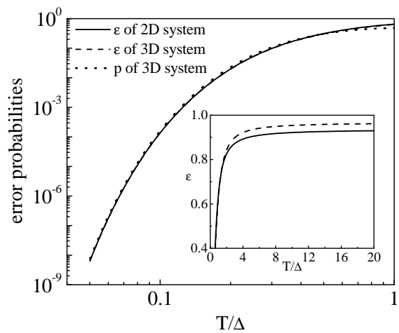
FIG. 3: Error probabilities \epsilon on a GHZ state and p on the cluster state as functions of the temperature. For 2D system the GHZ state is a four-qubit state, and for 3D system the GHZ state is a five-qubit state. \epsilon are almost the same for 2D and 3D systems when the temperature T < \Delta . When T/\Delta = 0.2 , p = 3\% , which means errors induced by a lower temperature are tolerable by using the topological error correction algorithm on the 3D system.
