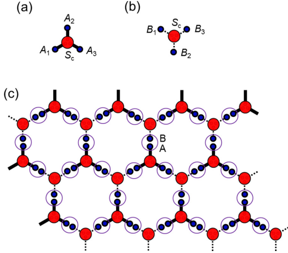
FIG. 1. (Color online) Illustration of bottom-up approach. Panels (a) and (b) illustrate the building block of one unit, which consists of one center spin-3/2 and three outer three virtual bond qubits. Two virtual bond qubits, each from a neighboring unit, form a physical bond spin-3/2 particle, as shown by circles enclosing them in (c). A two-dimensional or three-dimensional structure can be constructed.
