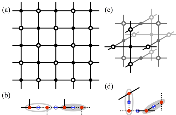
FIG. 3. (Color online) Lattices of cluster states and microscopic construction of qubits. Panel (a) is the 2D square-lattice cluster state, and (c) is the unit cell of the 3D bcc (body-center-cubic lattice) cluster state. Both could be constructed from trivalent lattices (with degree-3 nodes) using the modification as shown in (b) and (d), respectively, which converts a degree-4 node to combinations of degree-3 nodes; see also Ref. [27]. Note that with such a construction, (a) will be turned to a brick-wall structure equivalent to the honeycomb lattice shown in Fig. 1(c). See also Fig. 6 and the Appendix for the conversion. In (b) and (d), each logical qubit (oval) is composed of spins from two units. The spins inside each oval will eventually be converted to one logical qubit. The circle (which includes two virtual qubits, i.e., a single bond particle) between the two ovals is used to entangle neighboring two effective qubits (within the ovals) via measurement of a bond particle. Essentially, the product of two GHZ states from two such units can be converted to a single GHZ via local measurement on the bond particle inside the oval as well as one of the center particle.
