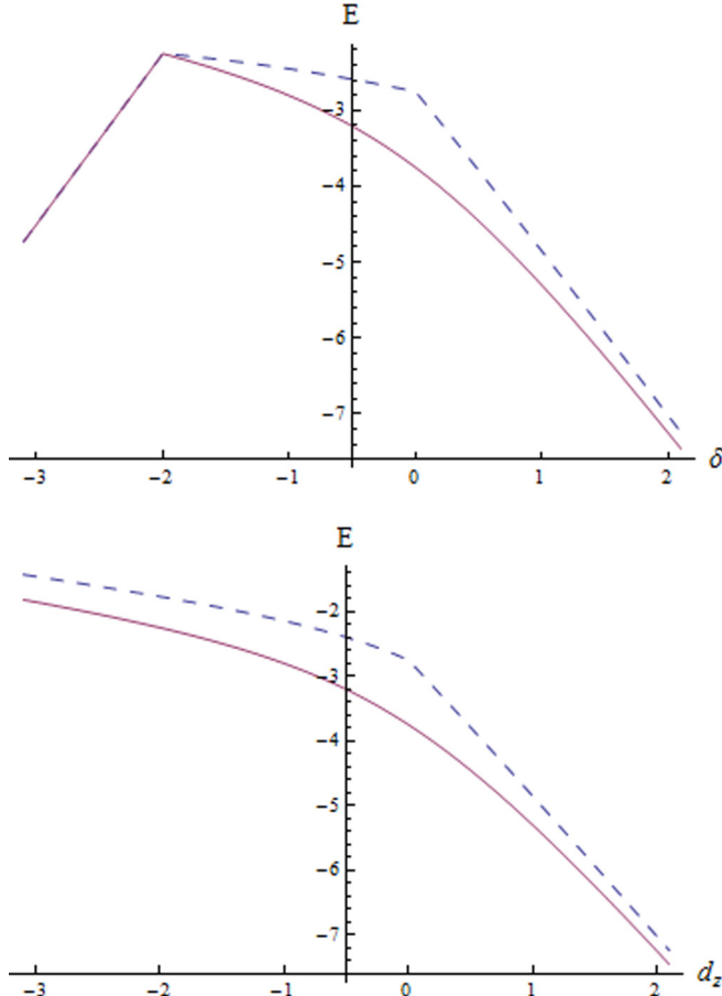
FIG. 2. (Color online) Ground-state and the first excited-state energies in each unit for the two models (top: model 1; bottom: model 2). The difference in the two energies is also the gap of the corresponding two- or three-dimensional models (for any finite system as well as in the thermodynamic limit). For the first model, the lowest two energy levels are degenerate for \delta \leq -2 . The ground-state energy exhibits discontinuity in its first derivative with respect to \delta , implying a first-order quantum phase transition in the model. However, for the second model, the ground-state energy is analytic for all range of d_z , implying nonexistence of phase transition.
