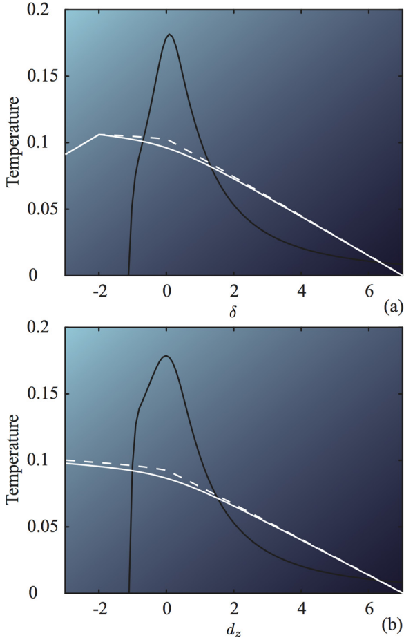
FIG. 5. (Color online) 3D phase diagrams in terms of computational power. (a) XXZ model; (b) anisotropic model. In the region below the solid black curve the equilibrium thermal states provide universal resource for MBQC. For reference, the energies for the ground state and the first excited is shown in white curves (solid and dashed, respective). Note that the transition temperatures are about three to four times higher than in two dimensions at the Heisenberg point.
