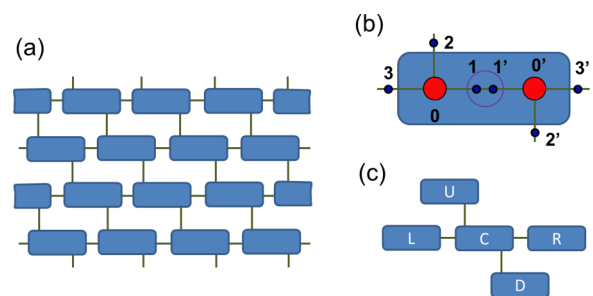
FIG. 6. (Color online) Generation of a cluster state on a square lattice: (a) original honeycomb (i.e., brick wall) lattice; (b) a block of spins that give rise to one logical cluster-state qubit; (c) a center logical block and its neighbor four blocks on a square lattice.
