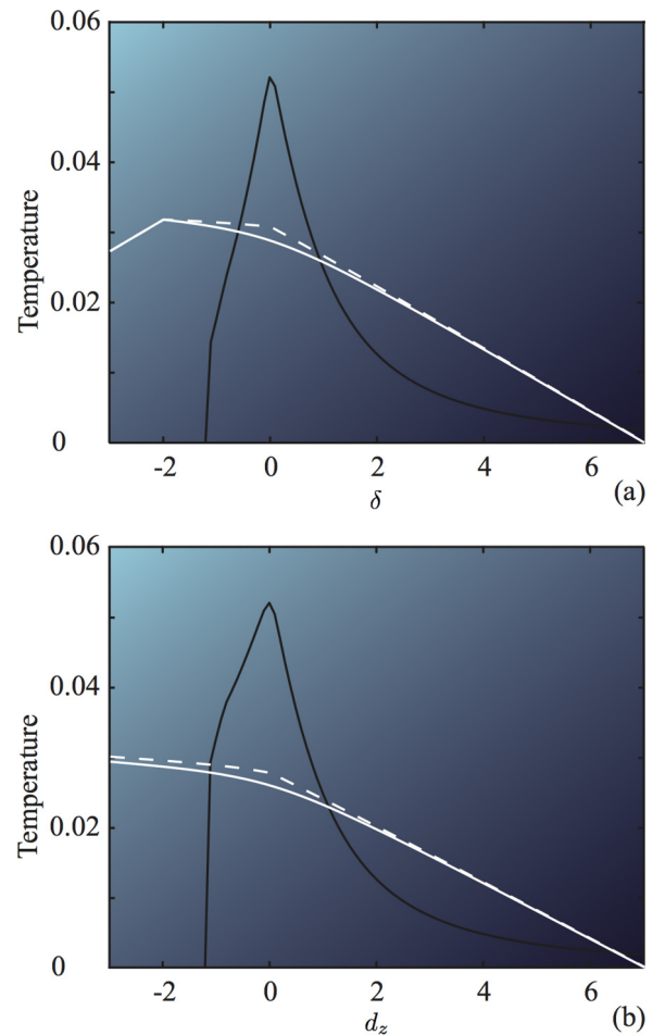
FIG. 4. (Color online) 2D Phase diagrams in terms of computational power: (a) Upper: the XXZ model; (b) bottom: the anisotropic model. In the region below the solid black curve the equilibrium thermal states provide universal resource for MBQC. For reference, the energies for the ground state and the first excited is shown in white curves (solid and dashed, respective).
