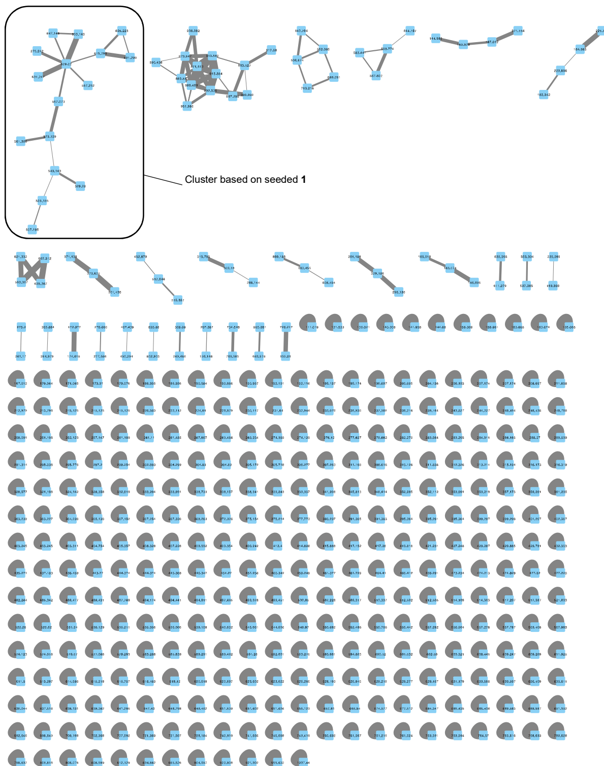
Figure 3. Molecular network of the extract obtained from TLT/PHB/001 generated using Cytoscape v3.5.1. (The Cytoscape Consortium, New York, USA).
