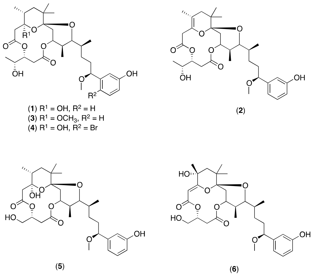
Figure 2. Chemical structures of alysiatoxin (4), and related analogues debromoaplysiatoxin (1), anhydrodebromoaplysiatoxin (2), 3-methoxydebromoaplysiatoxin (3), oscillatoxin A (5) and 31-noroscollatoxin B (6).
