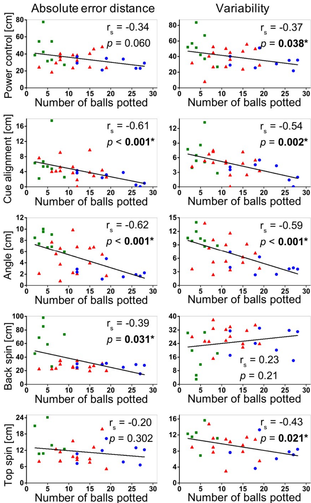
Figure 3. Correlations between 9-ball skill tests (absolute error distance and variability) and the 15-ball performance test (number of balls potted in best 2 out of 3 trials). The recreational group is shown in green squares; the university team is shown in red triangle; the national team is shown in blue dot.
