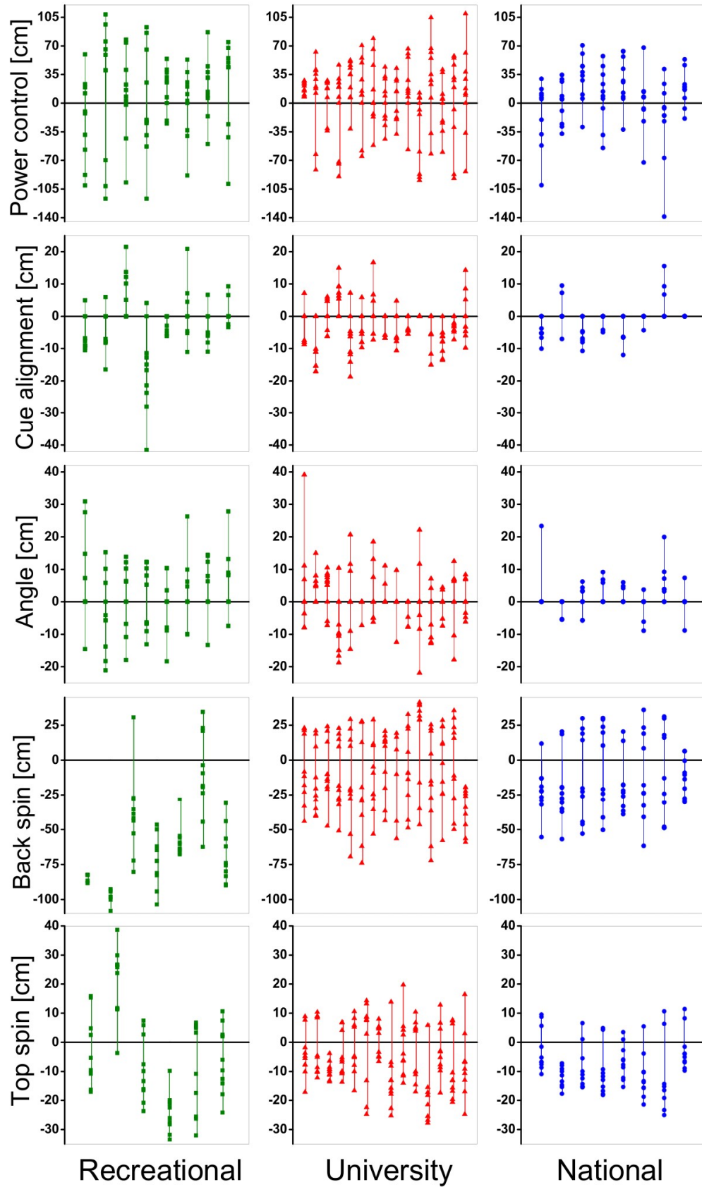
Figure 2. Error distances of 10 individual trials for each participant. The recreational group is shown in green squares; the university team is shown in red triangle; the national team is shown in blue dot.
