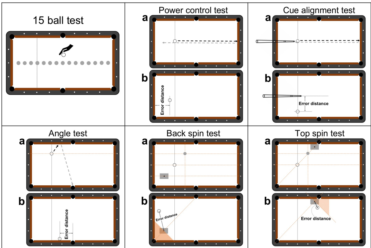
Figure 1. Scheme of the 15-ball test and 5 skills tests.
