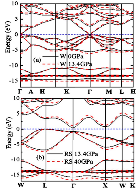
FIG. 4. (Color online) Band structure: (a) wurtzite InN under 0 and 13.4 GPa (b) rocksalt InN under 13.4 and 40 GPa.
