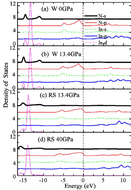
FIG. 5. (Color online) Density of states for N 2s , N 2p , In 5s , In 5p , and In 4d . (a) wurtzite InN under no-external-pressure conditions; (b) wurtzite InN under 13.4 GPa (c) rocksalt InN under 13.4 GPa, and (d) rocksalt InN under 40 GPa.
