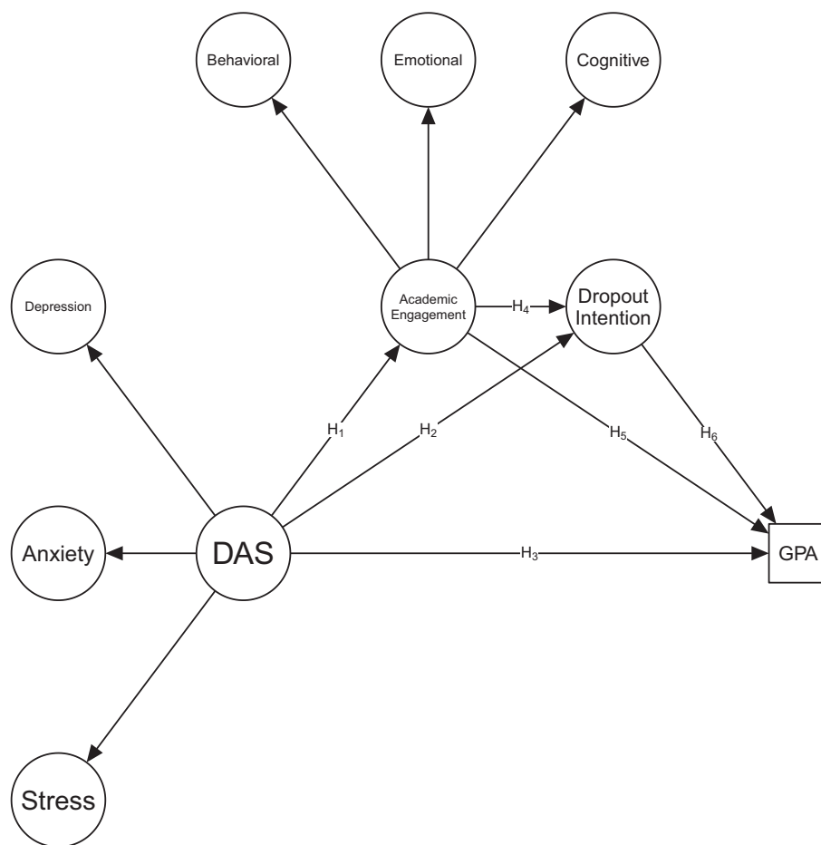
Fig. 1. Hypothesized model.
