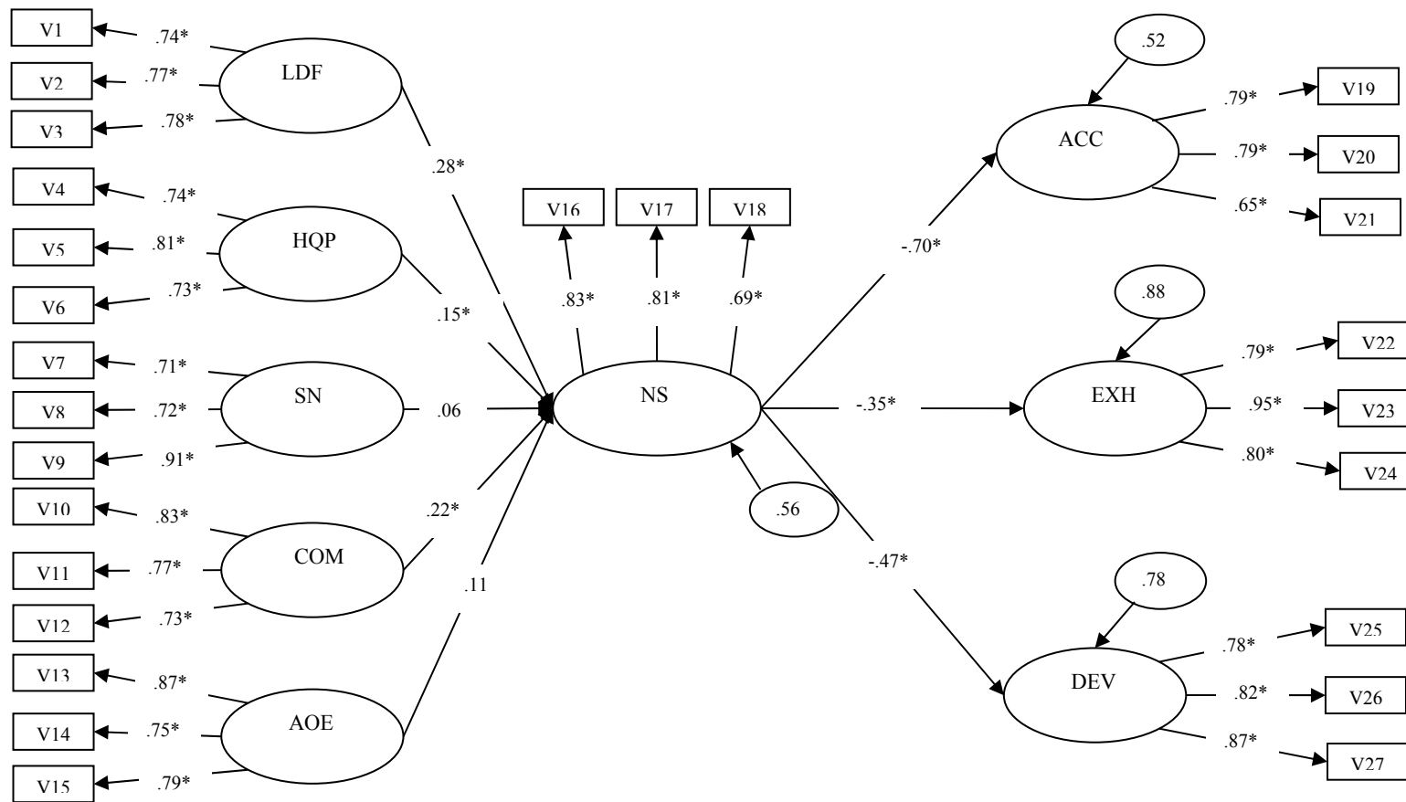
Figure 1. Standardized estimates for the full structural equation model.
